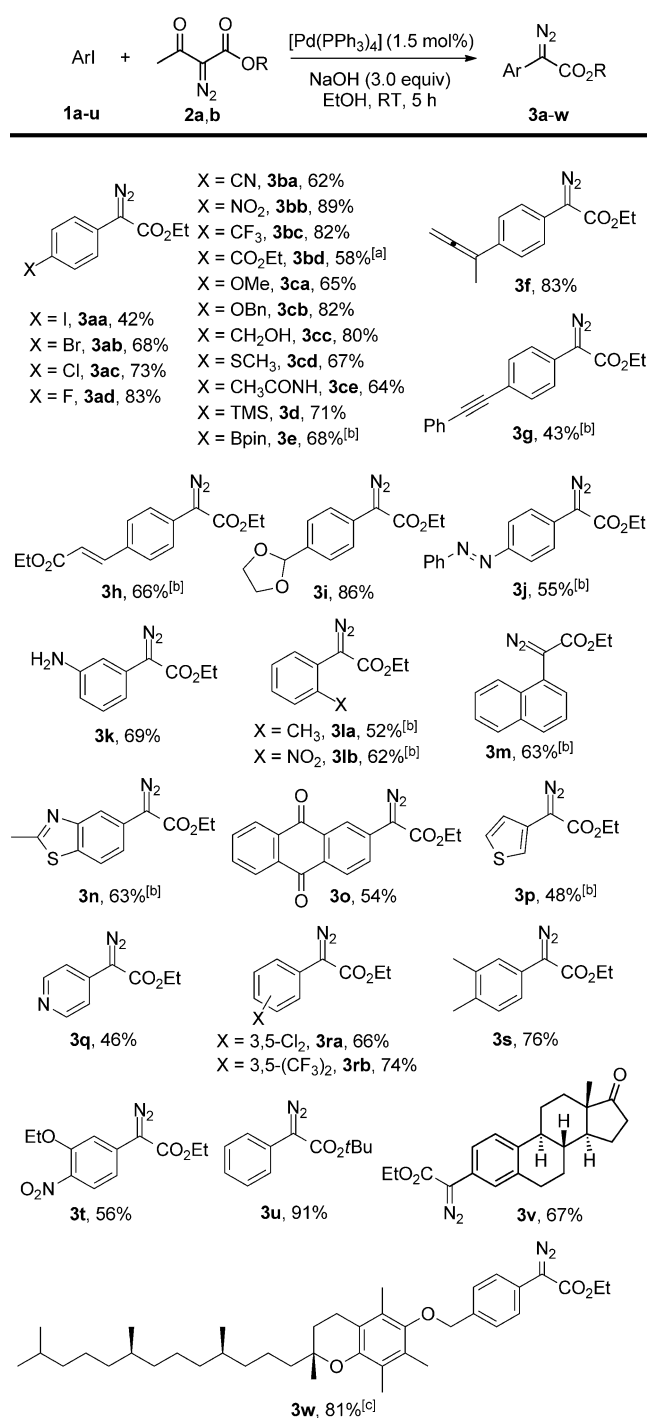
Scheme 2. Scope of the coupling reaction of acyldiazooacetate with aryl iodide. If not otherwise noted, the reactions were carried out with the aryl iodides 1a–u (0.25 mmol), acyldiazooacetate 2a,b (0.3 mmol), [\text{Pd}(\text{PPh}_3)_4] (1.5 mol %), NaOH (3.0 equiv) in EtOH (1 mL) for 5 h at room temperature. All the yields refer to products isolated after column chromatography. [a] The substituent X in the substrate is \text{CO}_2\text{Et} . [b] Used [\text{Pd}(\text{PPh}_3)_4] (5 mol %). [c] To enhance the solubility, petroleum ether (0.5 mL) was added. TMS = trimethylsilyl.
